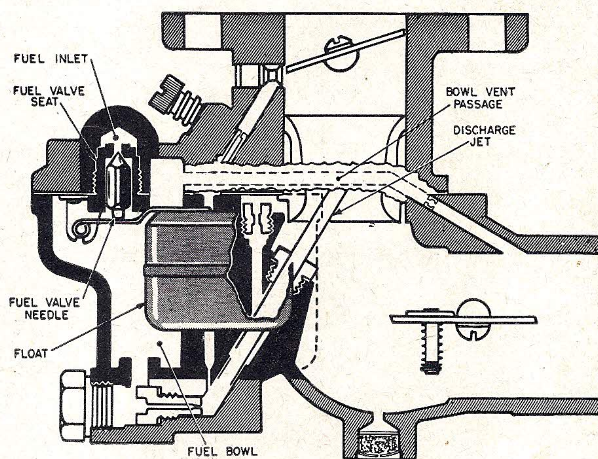
FUEL SUPPLY SYSTEM
