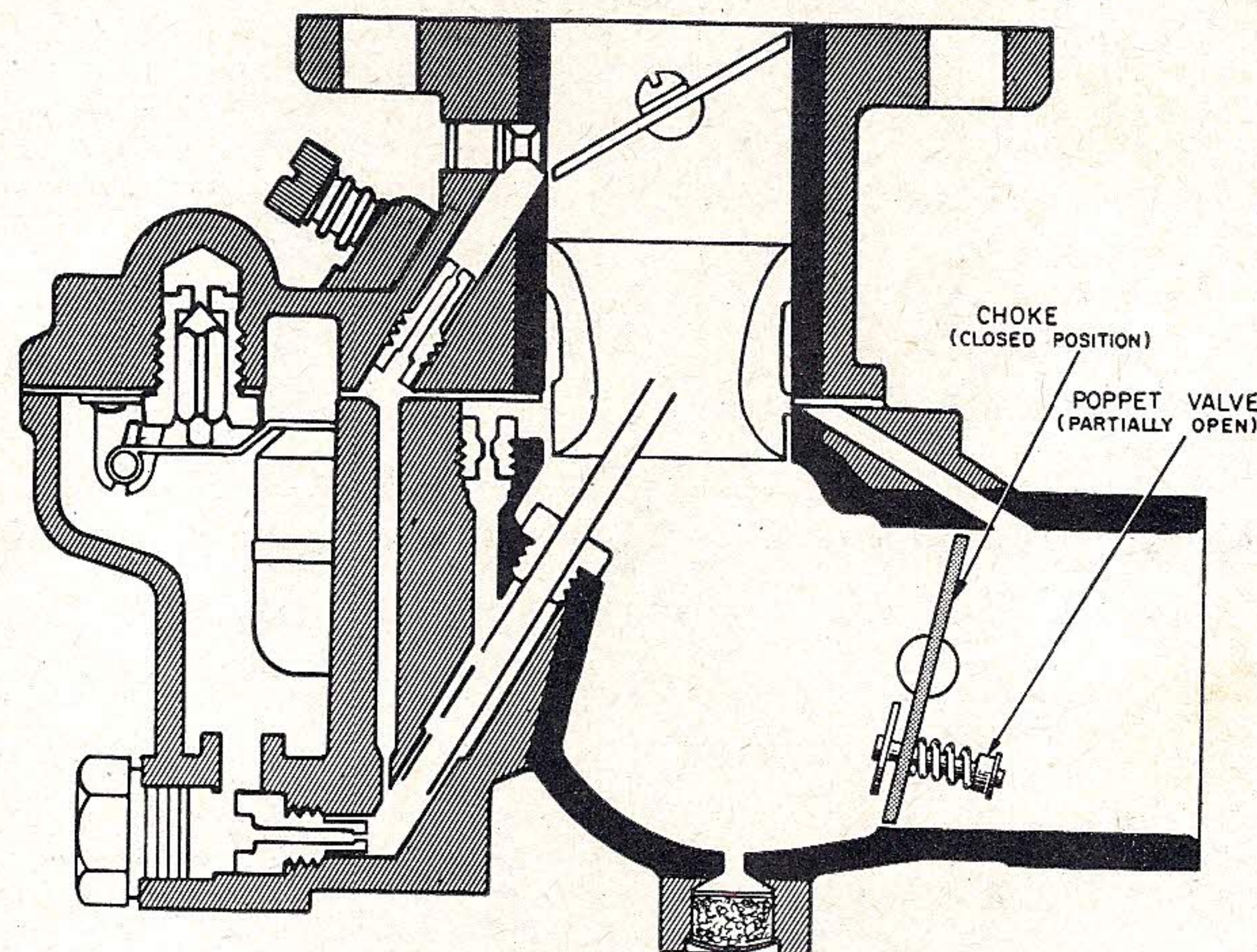
CHOKE SYSTEM
