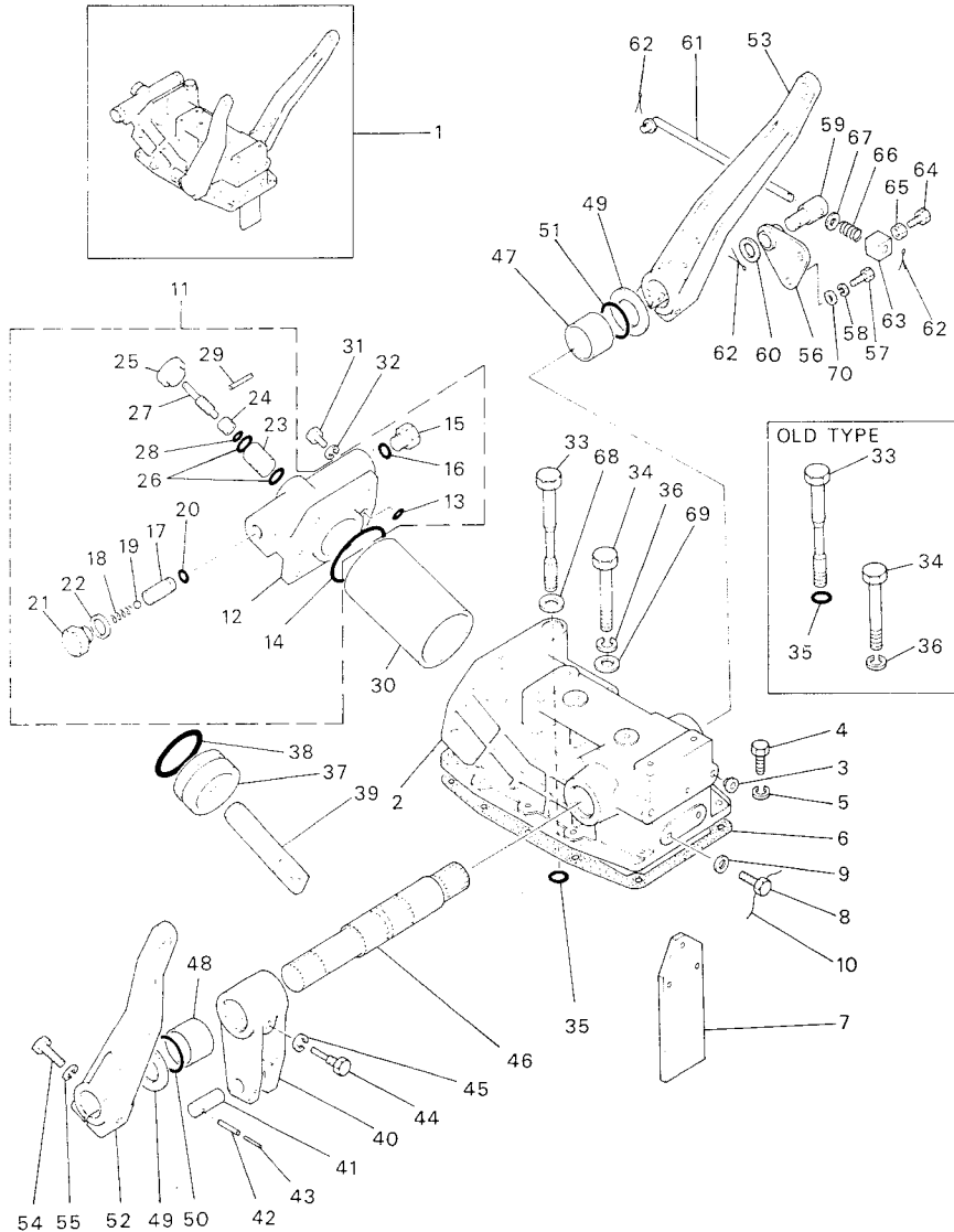
Fig. 58 HYDRAULIC LIFT
