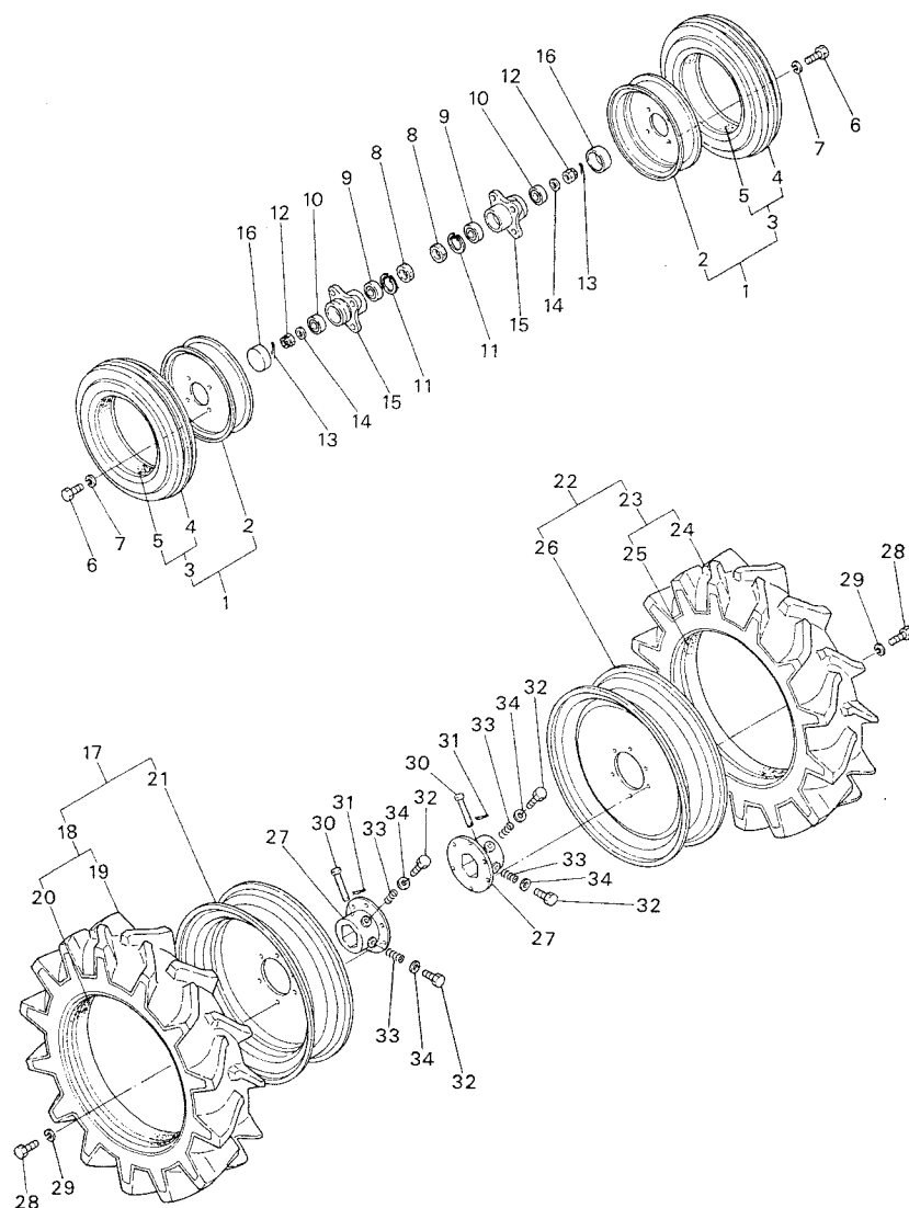
Fig. 50 FRONT &amp; REAR TIRES (U.S.A. &amp; S.AFRICA) [YM155]
