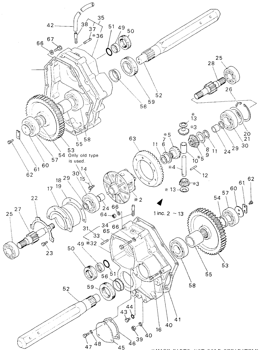
Fig. 43 REAR AXLE [YM135,YM135D]
