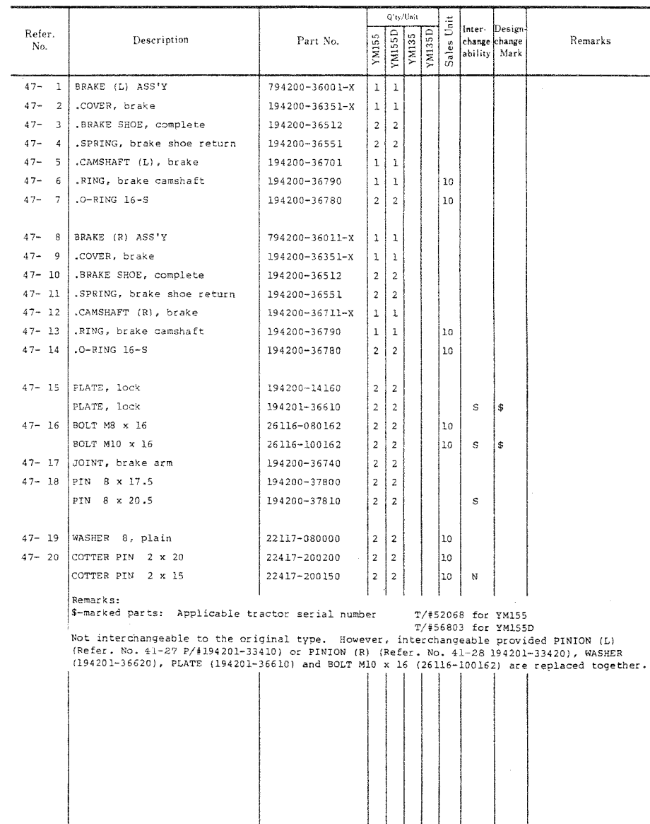
Fig. 47 BRAKES (EXCEPT PORTUGAL) [YM155,YM155D]
