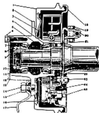
FIG. 13—WHEEL BEARING
