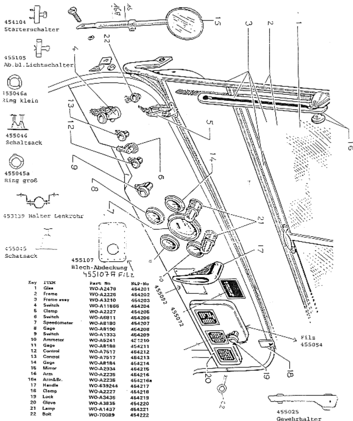
Front compartment and instrument panel
