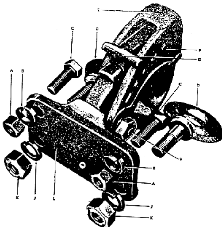
Pintel assembly Page 44
