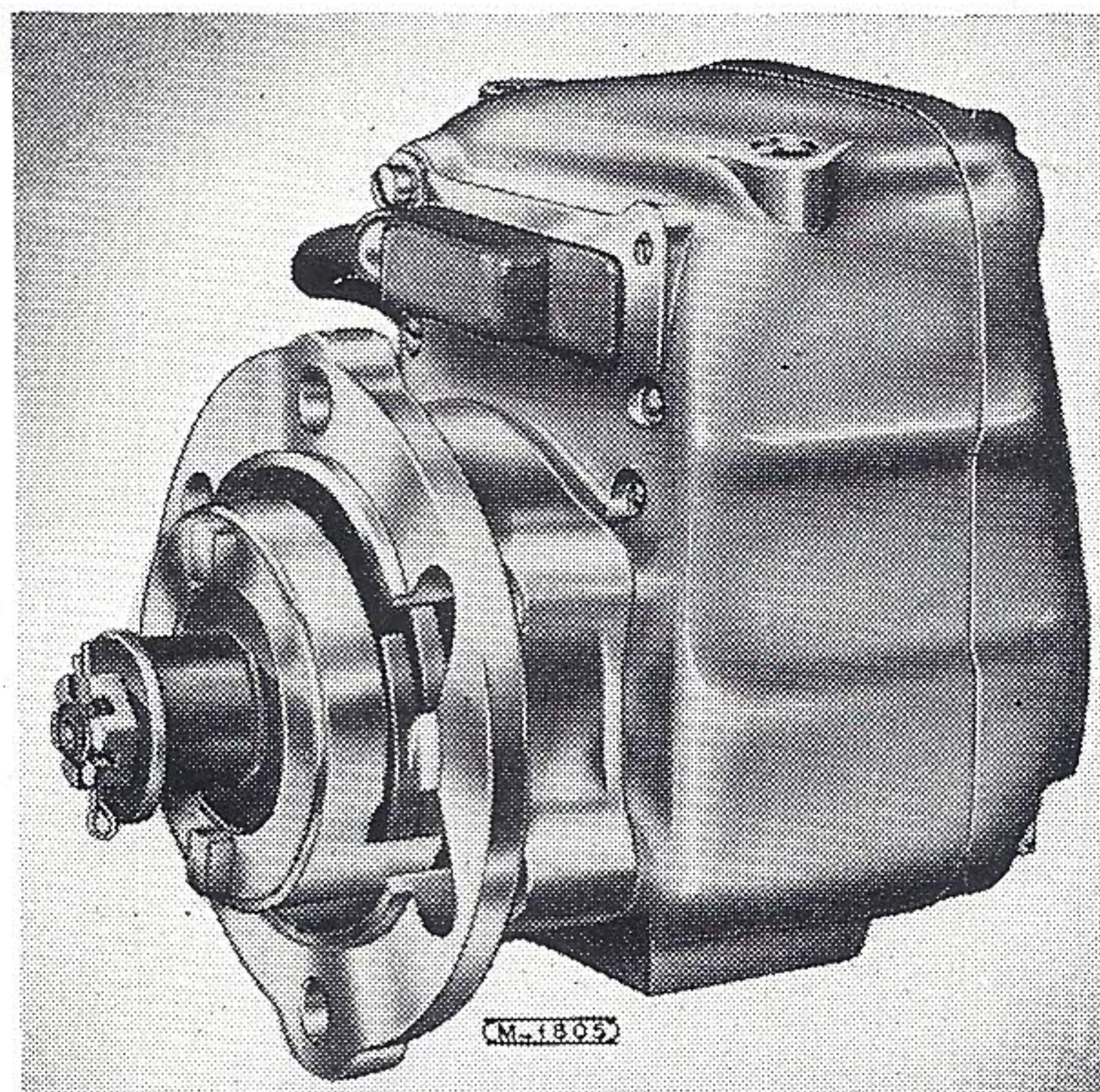
Typical Flange Mounted "H" Series Magneto
