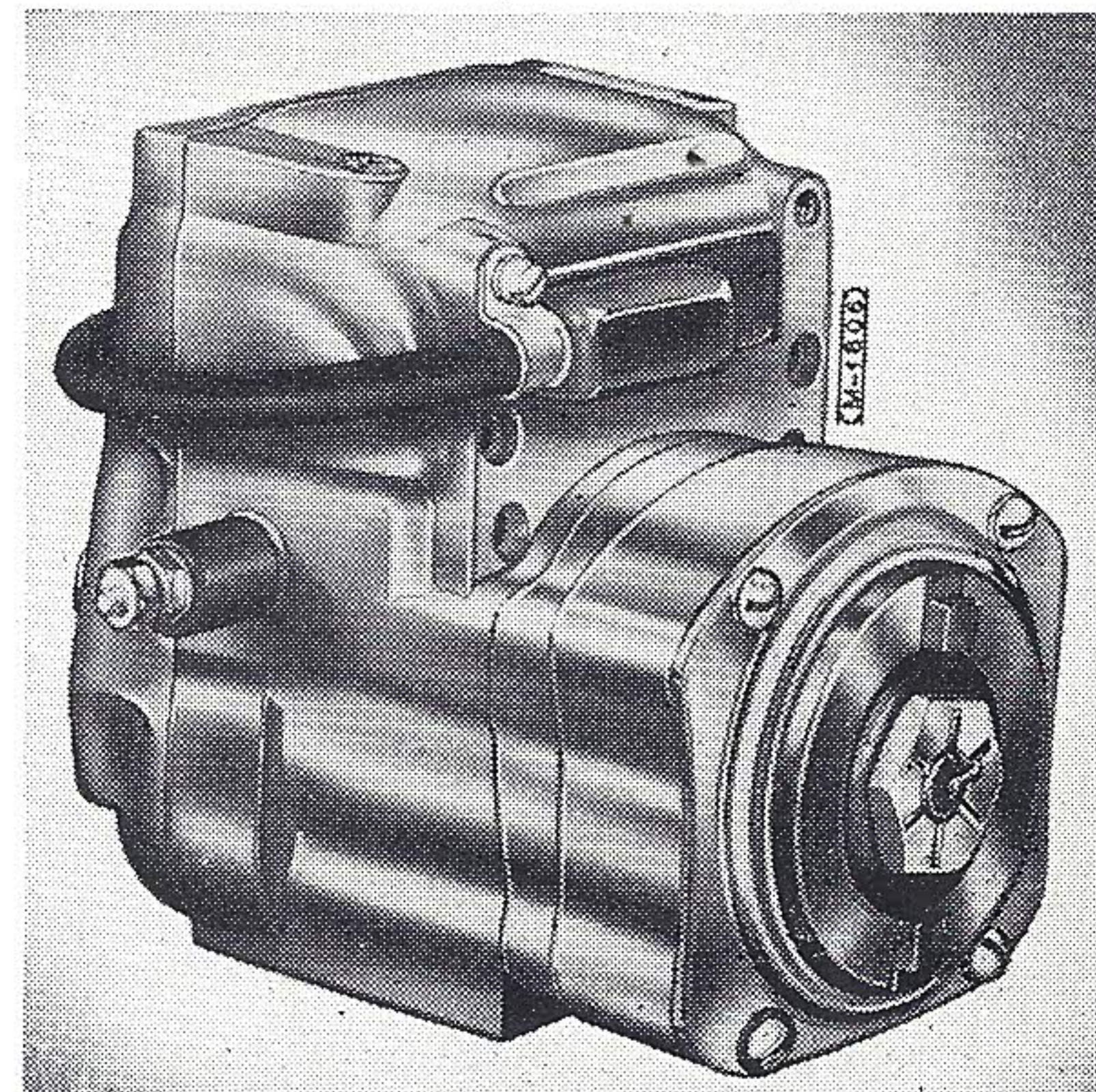
Typical Base Mounted "H" Series Magneto
